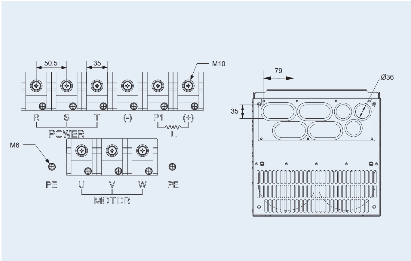
d) Applies to RNB2110 ~ RNB2132
