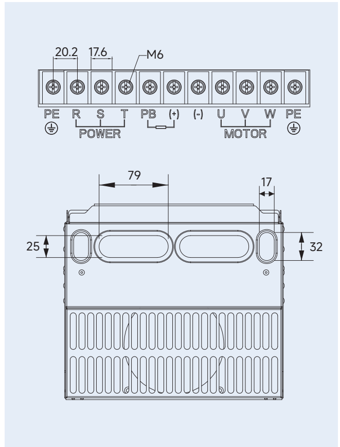
b) Applies to RNB2030 ~ RNB2037
