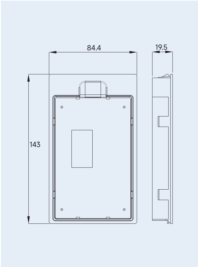
b) Panel bracket dimensions
