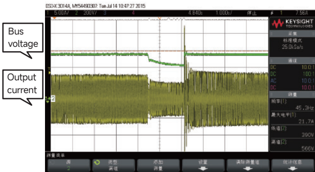
Undervoltage adjustment
