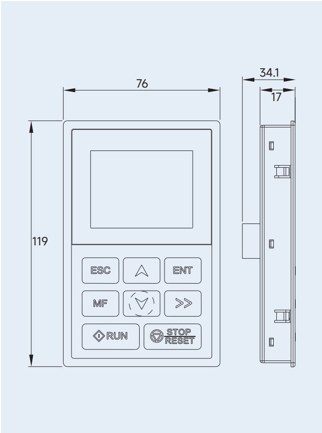
a) Panel dimensions
