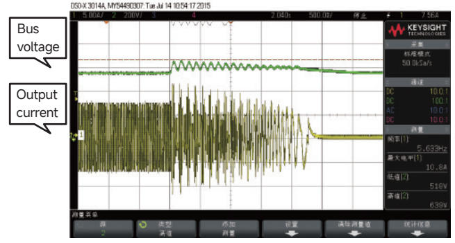
Overvoltage suppression
