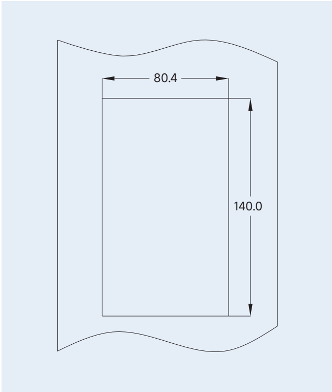
d) Panel bracket cutout dimensions
