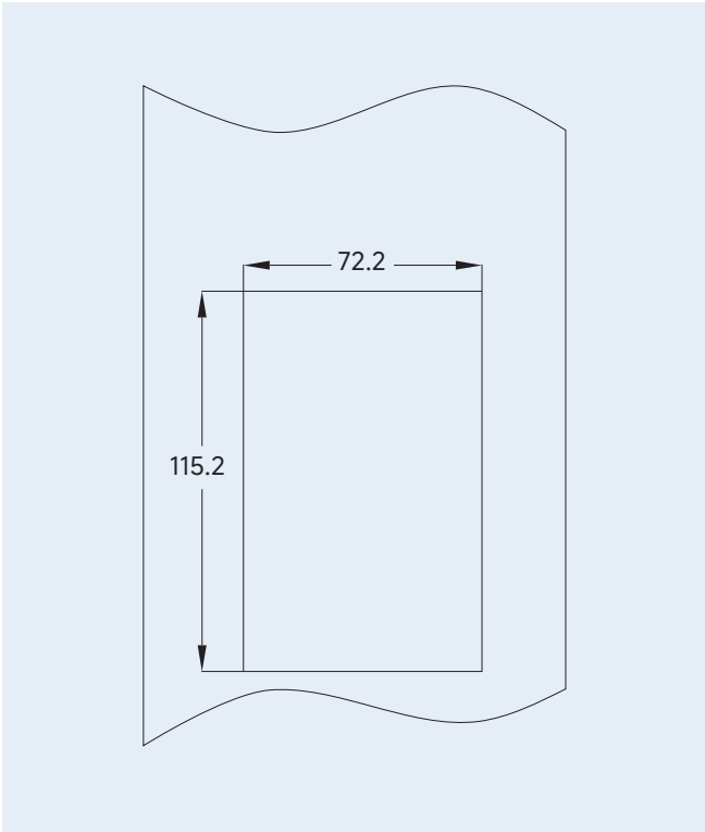
c) Panel cutout dimensions
