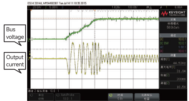
Overcurrent stall protect function
